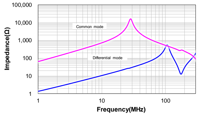
VCRHC1210-220M
