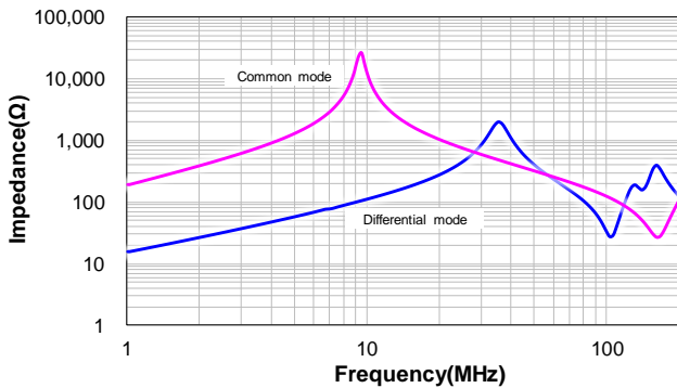
VCRHC1210-330M
