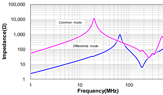
VCRHC1210-150M
