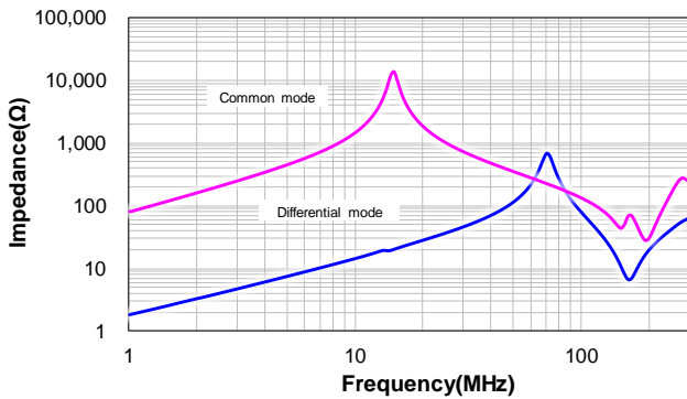
VCRHC1210-330M
