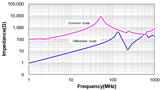
VCRHC1210-100M
