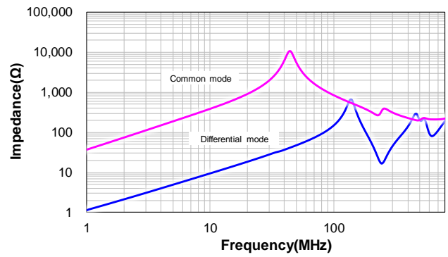
VCRHC1210-120M
