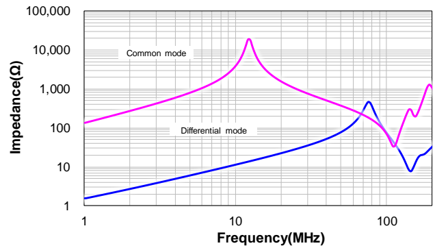
VCRHC1210-470M
