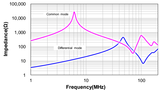
VCRHC1210-470M
