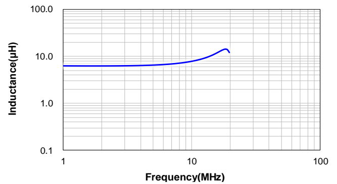
CSUC1514-6R8M:6R8M
