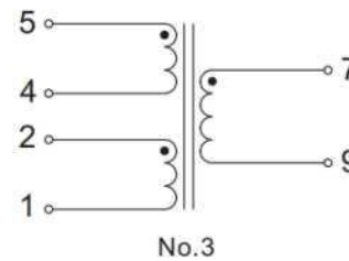
Double Input / Single Output
