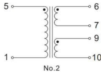
Single Input / Double Output
