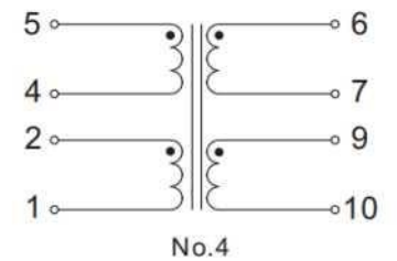
Double Input / Double Output
