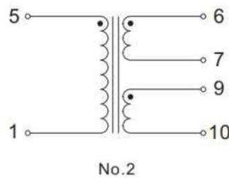
Single Input / Double Output
