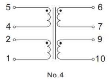
Double Input / Double Output
