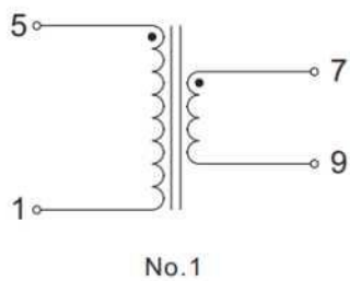
Single Input / Single Output
