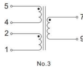
Double Input / Single Output
