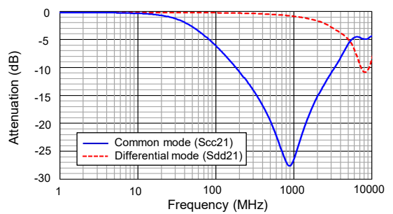
[ Attenuation characteristics ]
