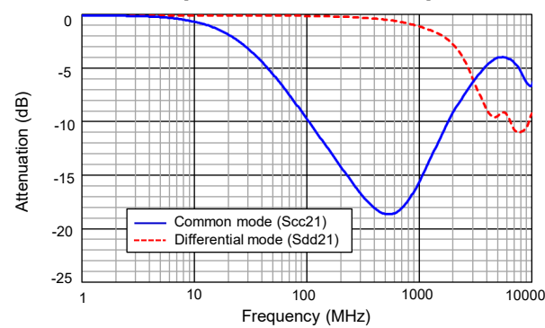
[ Attenuation characteristics ]
