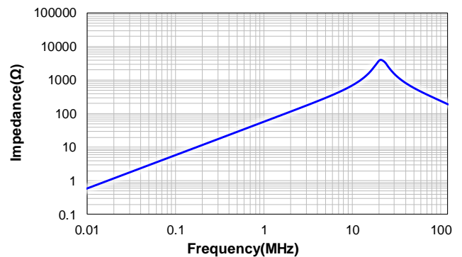
CSBX1812-100M
