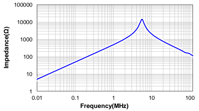
CSBX1812-820M
