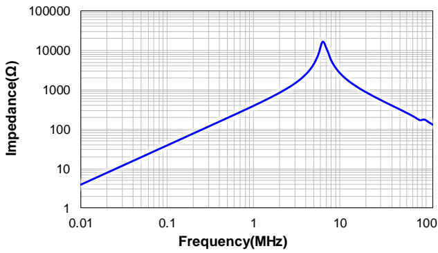
CSBX1812-650M
