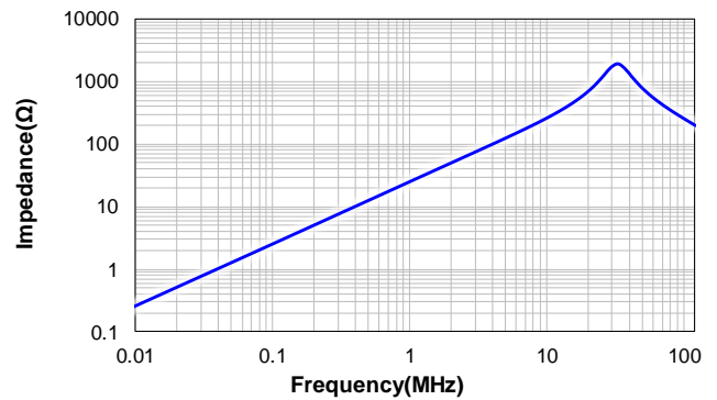
CSBX1812-6R8M
