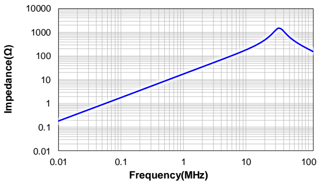
CSBX1812-5R3M
