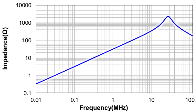
CSBX1812-8R2M
