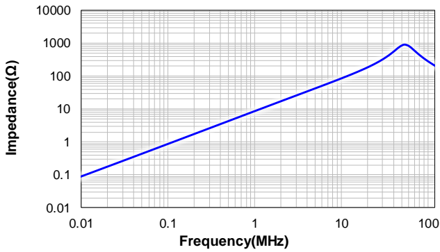
CSBX1812-3R0M
