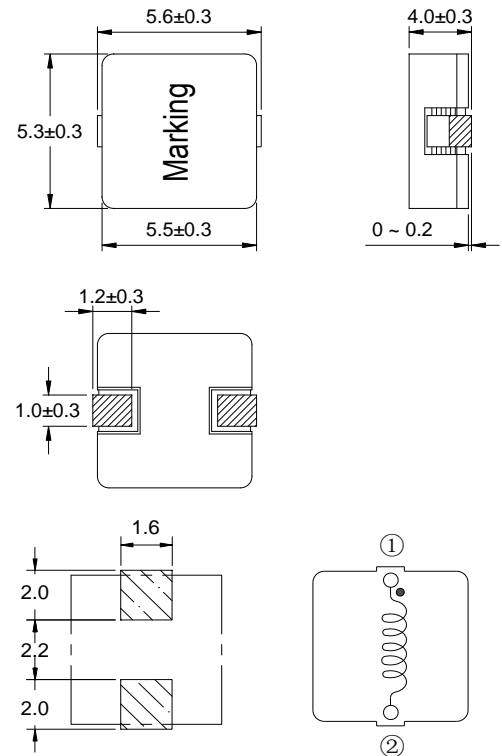
Typical Land Pattern
