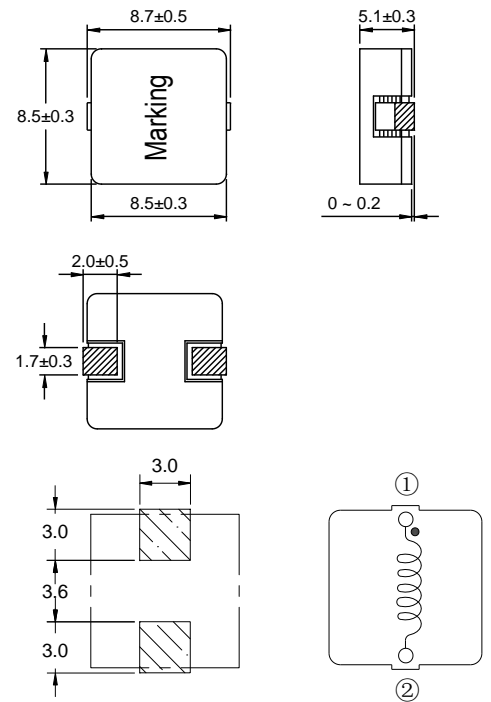
Typical Land Pattern
