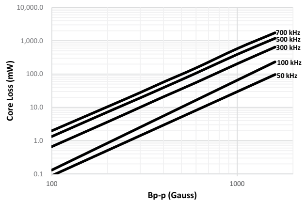
HCM1A0805V2-R47-R
