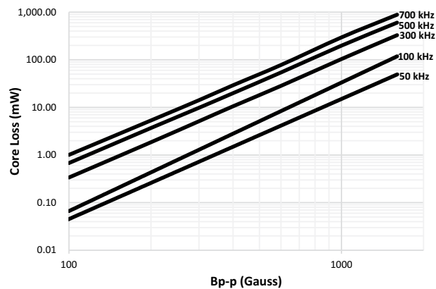
HCM1A0805V2-1R0-R
