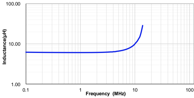
VSAB1365-6R8M
