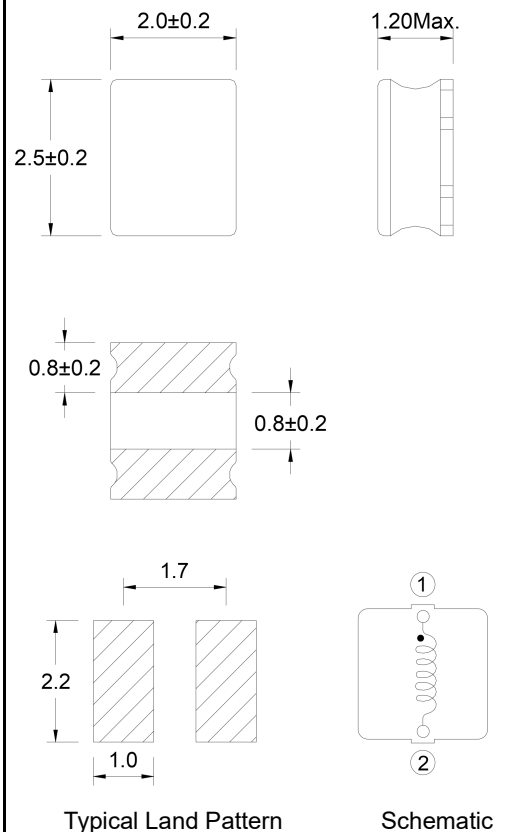
Typical Land Pattern
