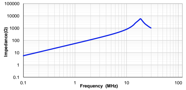
CSHB0415-100M
