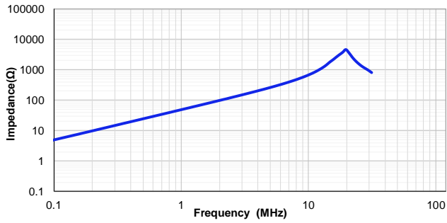
CSHB0415-8R2M
