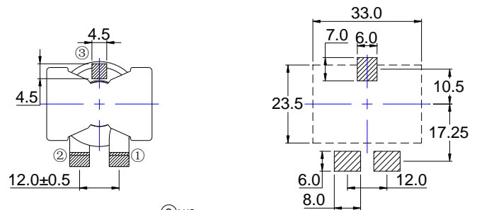
Reference Land Pattern
