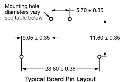
Typical Board Pin Layout
